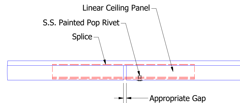
DETAIL A
