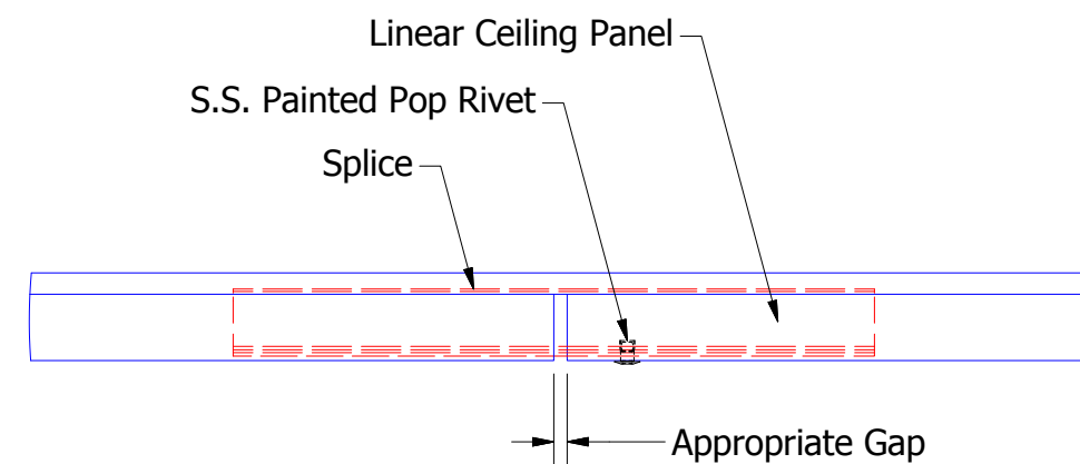
DETAIL A
