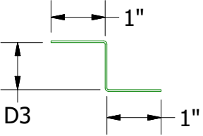
Support Z DWA681: D3 = 1" DSA681: D3 = 1 5/8"
