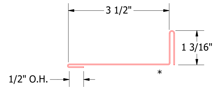
VLA620 - Outside Corner Receiver Strip
