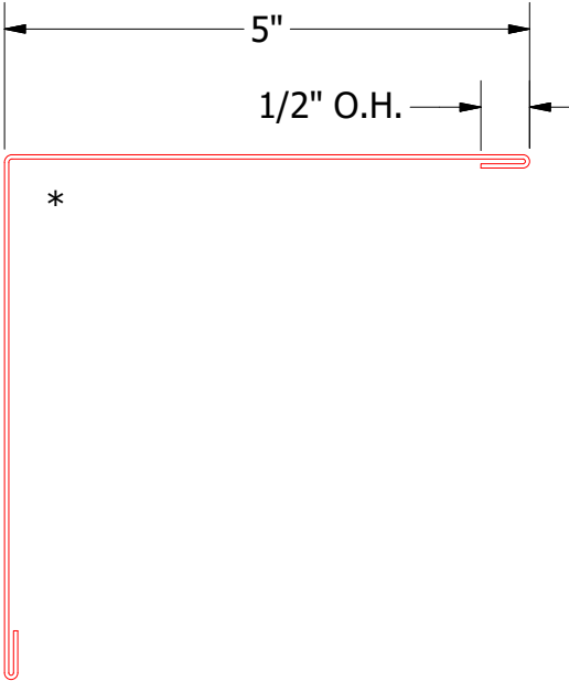
VLA600 - Inside Corner Cap
