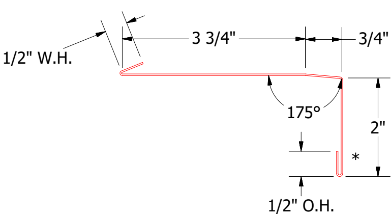
VLA670 - Window Sill Trim
