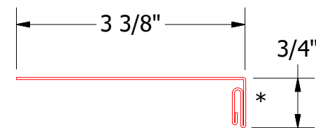
VLA039 - Snap J Base
