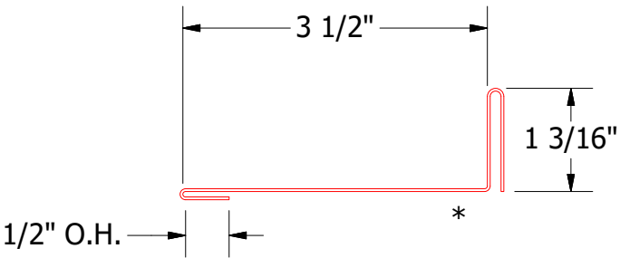
VLA620 - Outside Corner Receiver Strip
