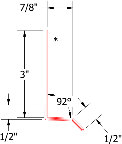
VLA661 - Base Trim
