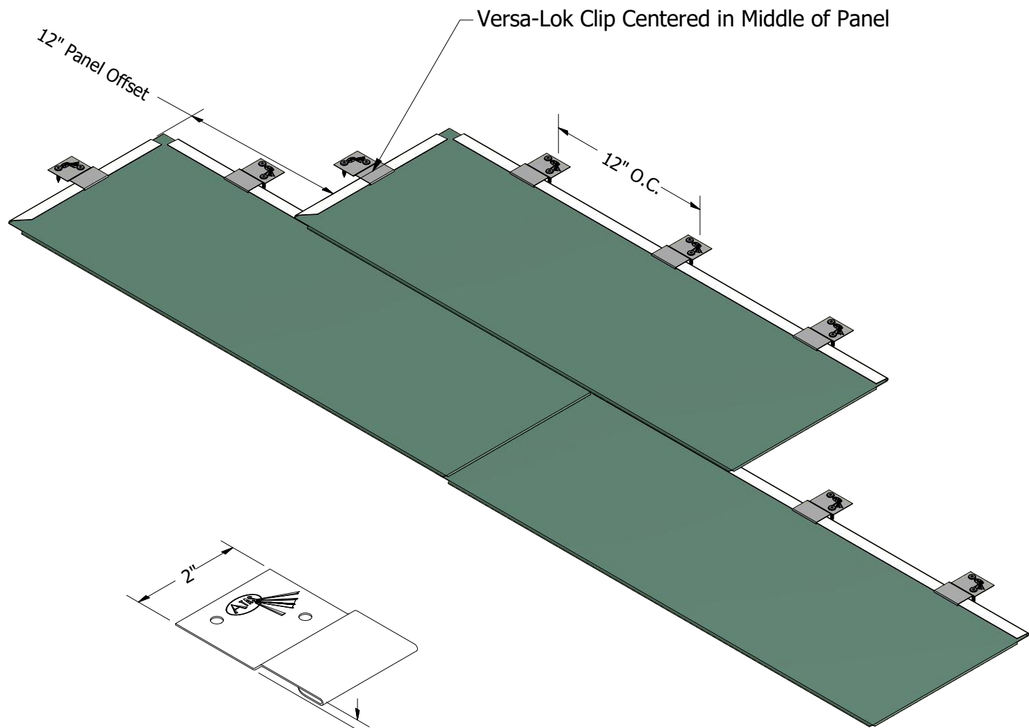
Horizontal Installation
