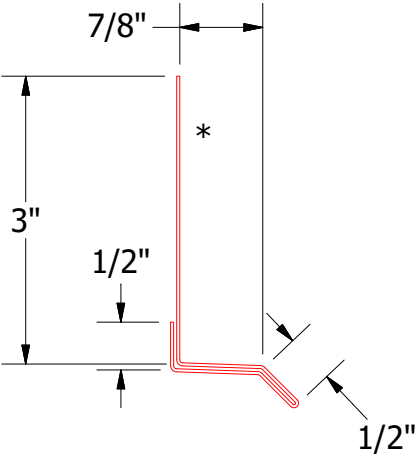
VLA661 - Base Trim
