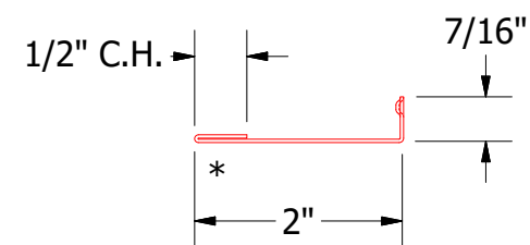
UNS200 - Snap J Cover
