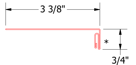
VLA039 - Snap Base
