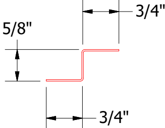
VLA681 - Support Z
