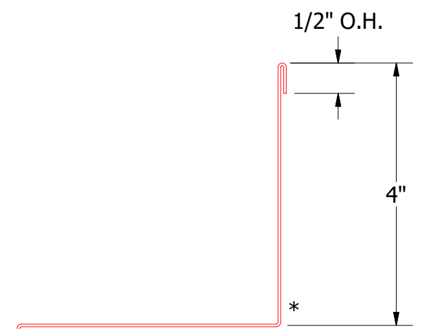
VLA610 - Outside Corner Cap
