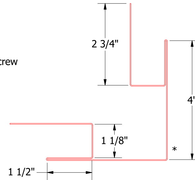
HCA602 - Outside Corner Post
