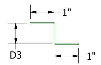
Support Z DWA681: D3 = 1" DSA681: D3 = 1 5/8"
