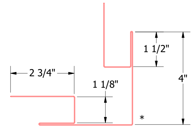
VSA602 - Outside Corner Post
