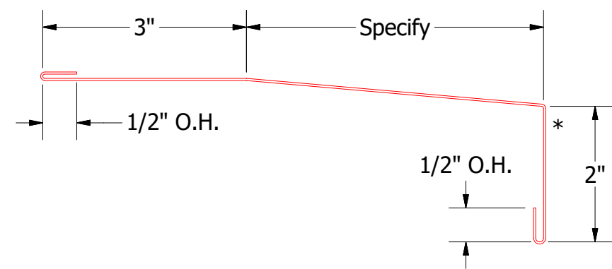
Window Sill Trim
