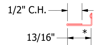
UNS078 - Snap J Cover
