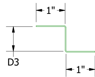
Support Z DWA681: D3 = 1" DSA681: D3 = 1 5/8"
