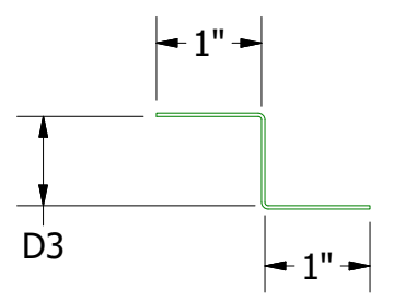
Support Z DWA681: D3 = 1" DSA681: D3 = 1 5/8"
