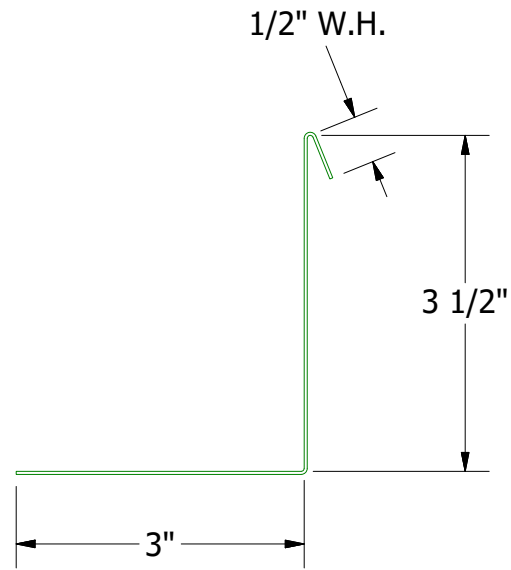
Angle Trim with Return (field fabricated from flat stock)
