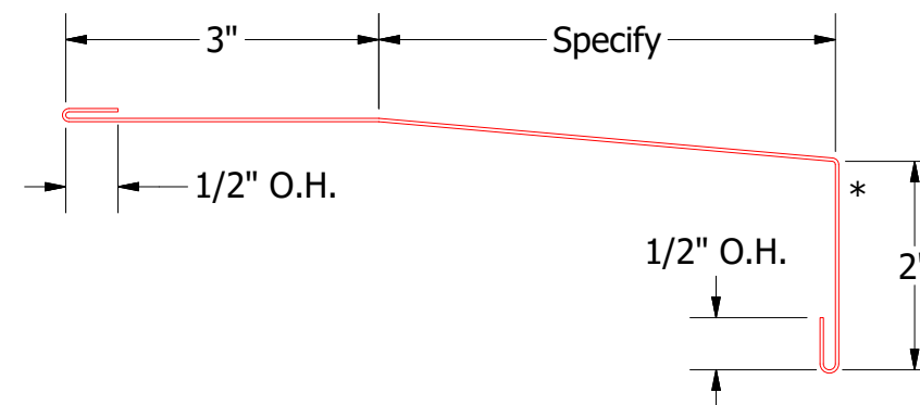
Window Sill Trim
