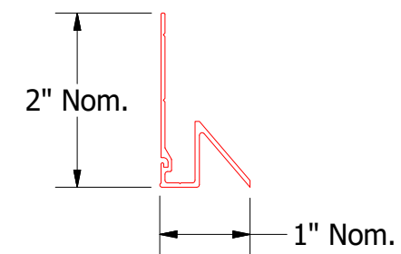
Drip Cap Extrusion
