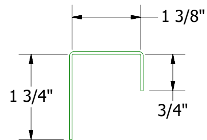
J Support
