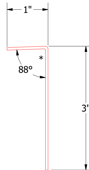
Coping Trim
