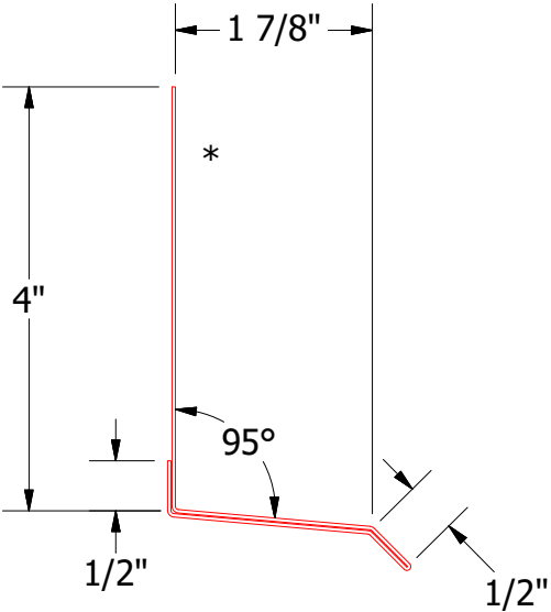
Base Trim
