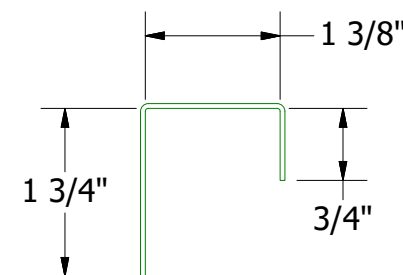
J Support
