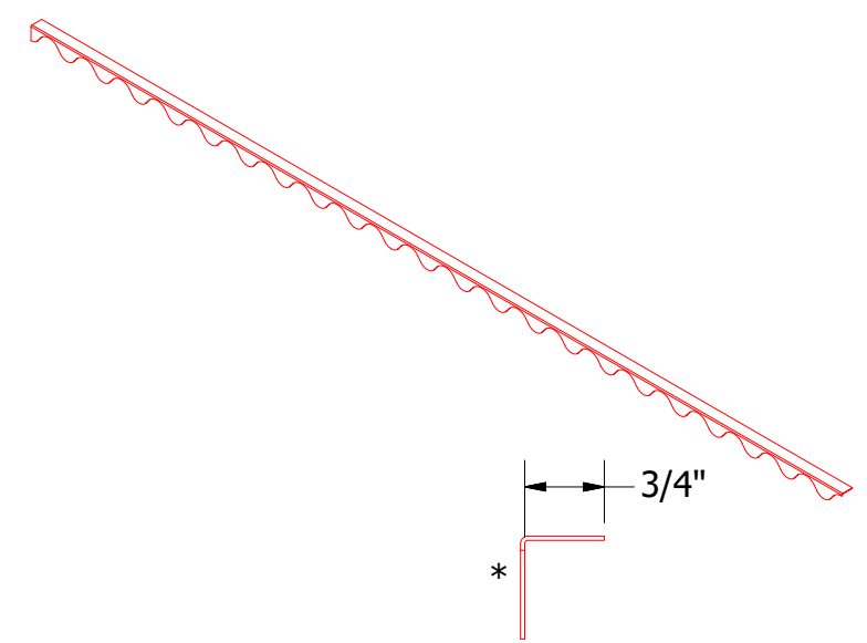
Metal Closure Angle
