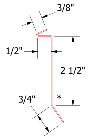
Counterflashing
