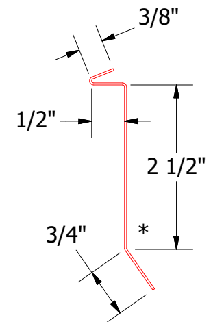
Counterflashing
