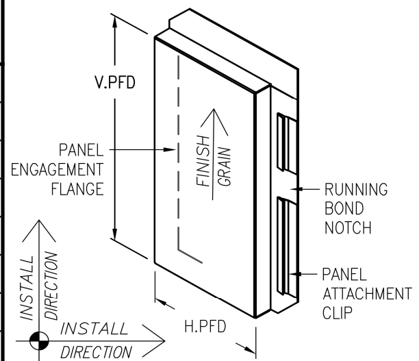
VERTICAL PANEL
