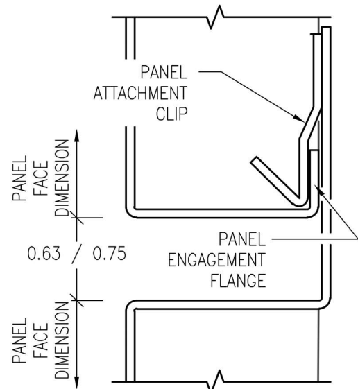
REVEAL SECTION
