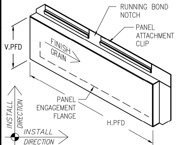
HORIZONTAL PANEL
