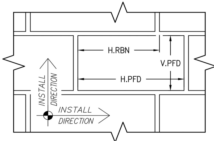
HORIZONTAL RUNNING BOND NOTCH
