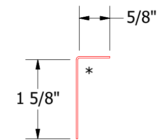
OPA680 - Angle Trim
