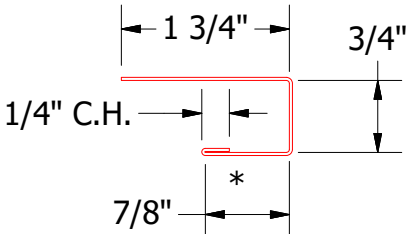
J Channel
