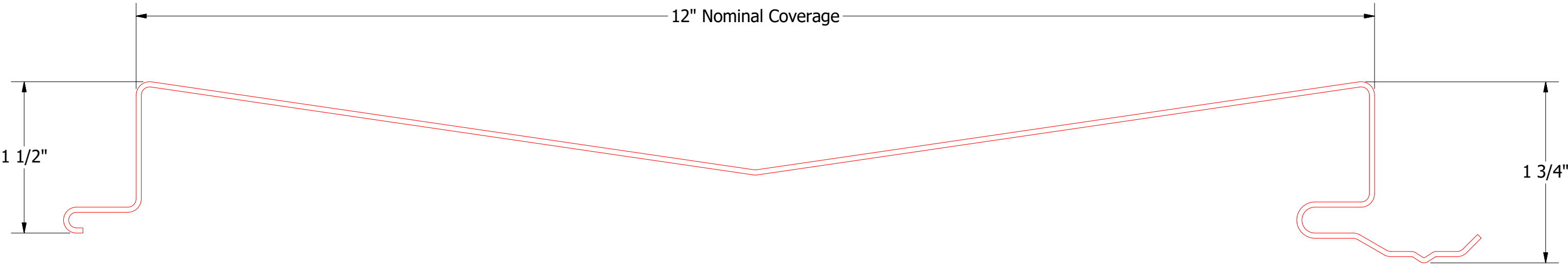
DSV120 Wall Panel
