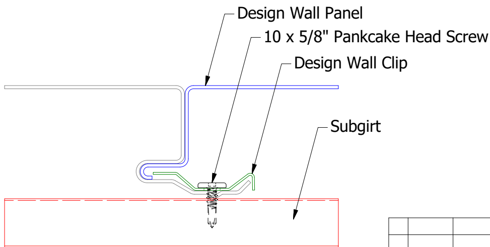
DETAIL A
