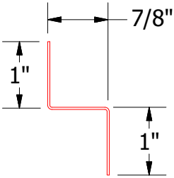
VSA681 - Support Z
