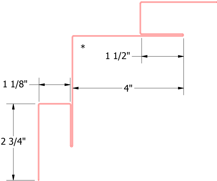
VSA601-Inside Corner Post
