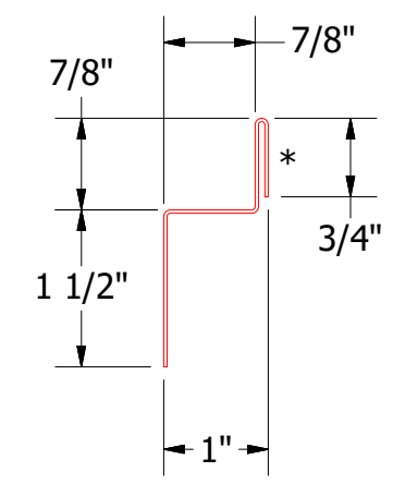
Top Trim
