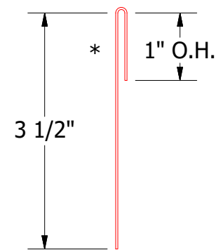
VSA962 - Utility Cleat without Return
