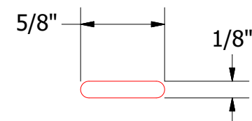
Fastener Slot
