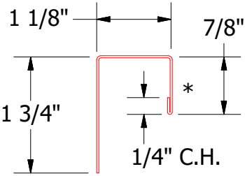
VSA118 - J Channel
