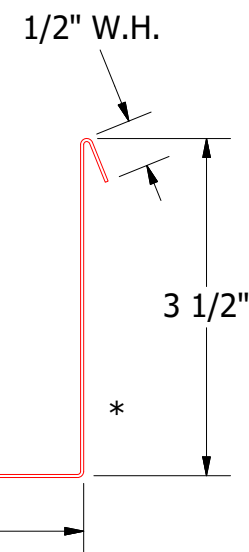
VSA683 - Angle Trim With Return
