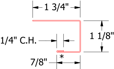
VSA118 - J Channel
