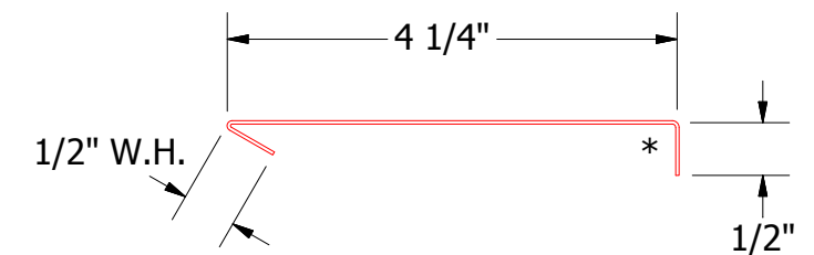
VSA690 - Head Angle Trim
