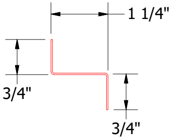
Z Closure
