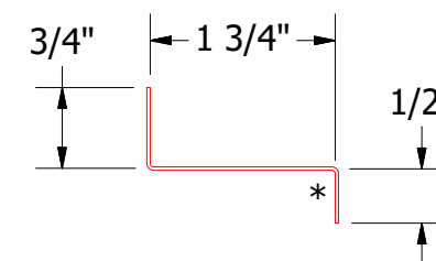
Z Closure
