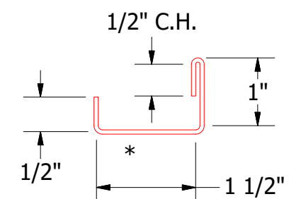
Panel Trim
