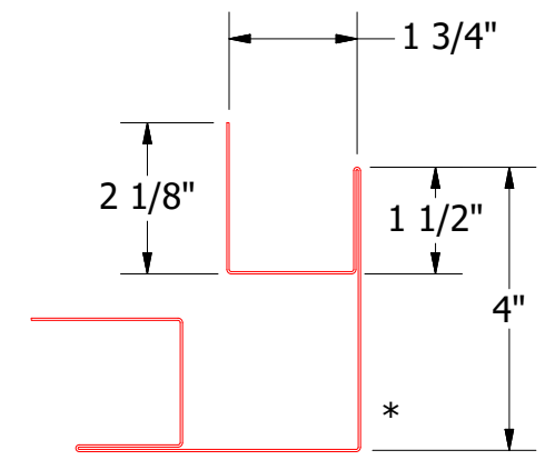
Outside Corner Post
