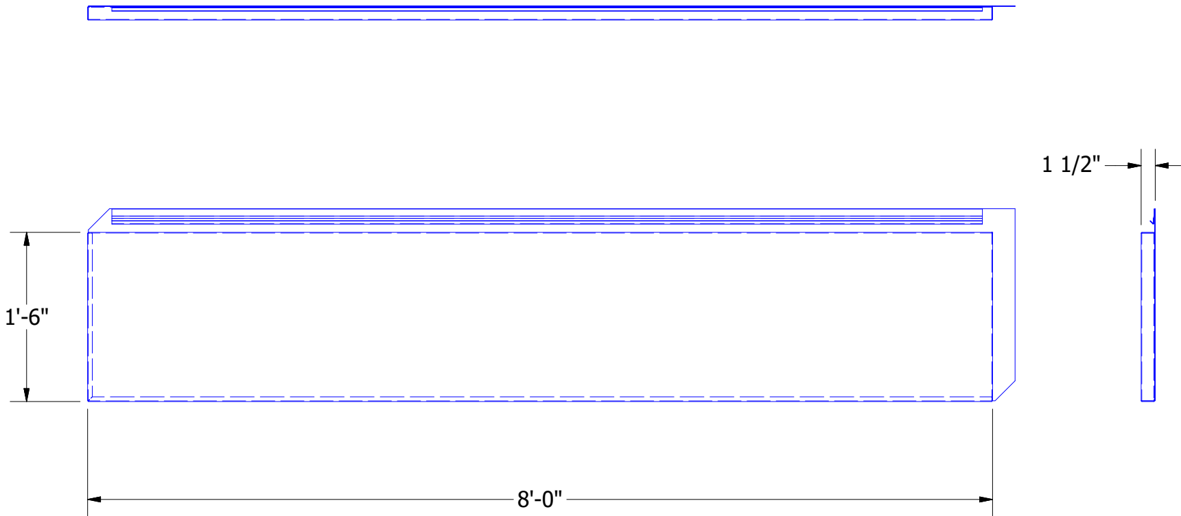
Omawall Horizontal Panel
