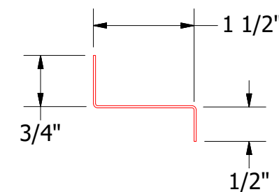
Window Sill Closure Trim
