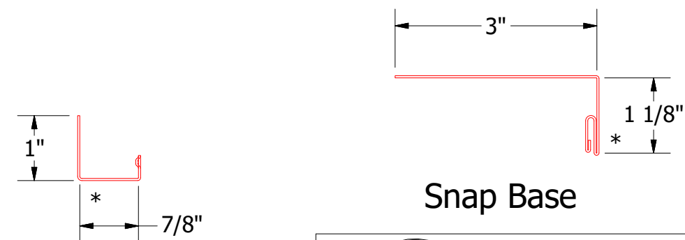
Snap Cover
