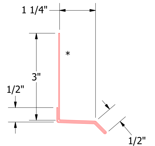
Base Trim
