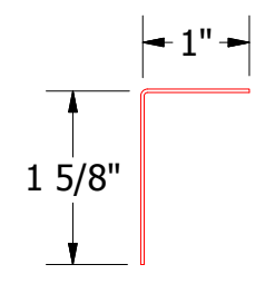
MCA680 - Angle Trim
