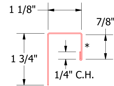
VSA118 - J Channel
