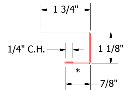
J Channel
