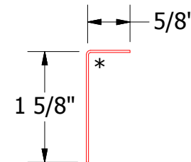
BGA680 - Angle Trim
