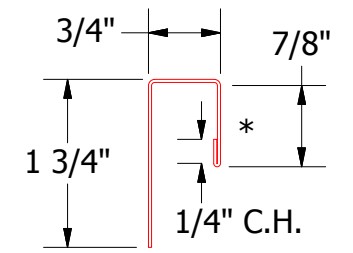
MFA034 - J Channel
