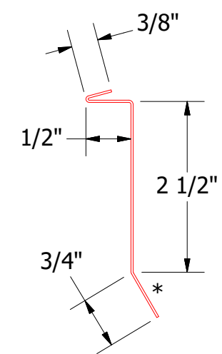
SCA980-Counterflashing
