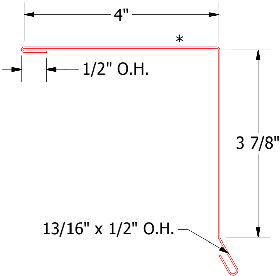
Gable Trim Cap
