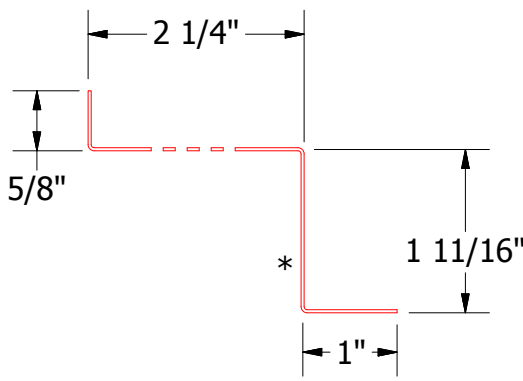
Vented Z Closure
