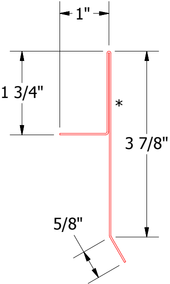
Gable Trim Starter Cleat
