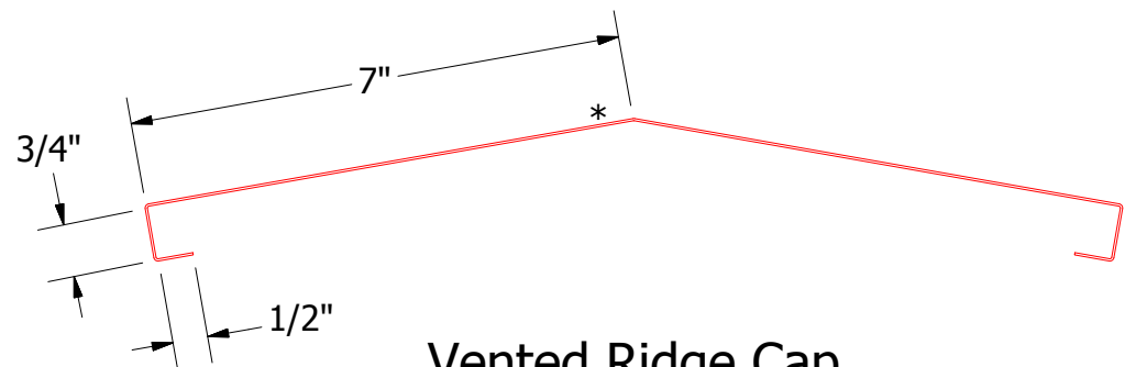
Vented Ridge Cap
