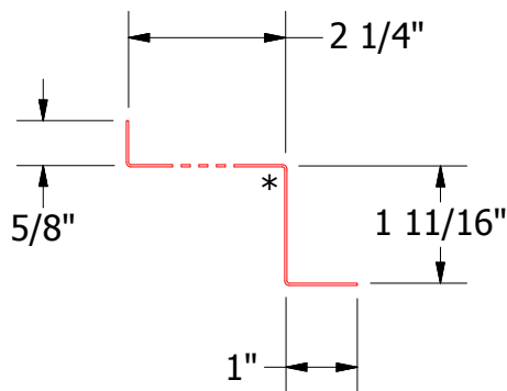
Vented Z Closure
