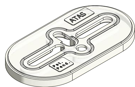
ASV Shim
