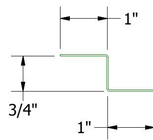
MCA681-Support Z
