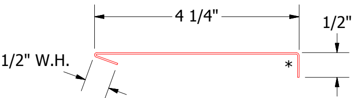
MCA690-Head Angle Trim
