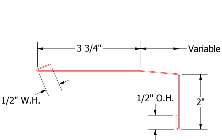
MCA670-Window Sill Trim
