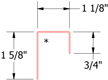
MCA270-J Closure
