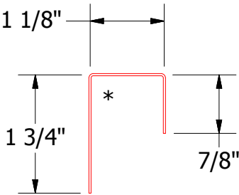
MCA118-J Channel
