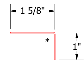
MCA680-Angle Trim
