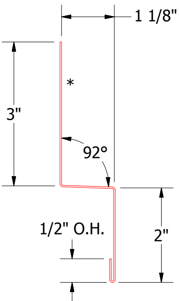
MCA550-Head Trim
