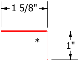
MCA680-Angle Trim
