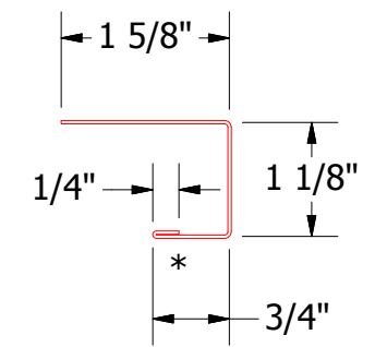
MCA118-J Channel
