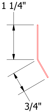
MFA995-Starter Cleat
