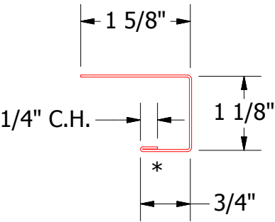
MCA118-J Channel
