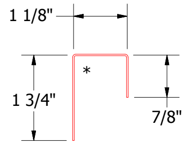
MCA118-J Channel
