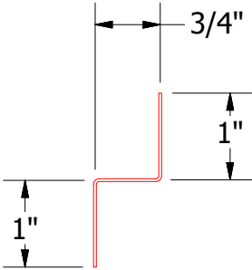
MCA681-Support Z
