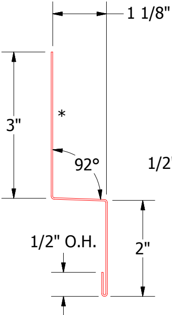
MCA550-Head Trim
