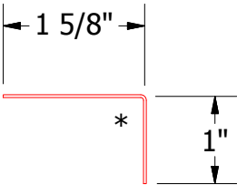
MCA680-Angle Trim
