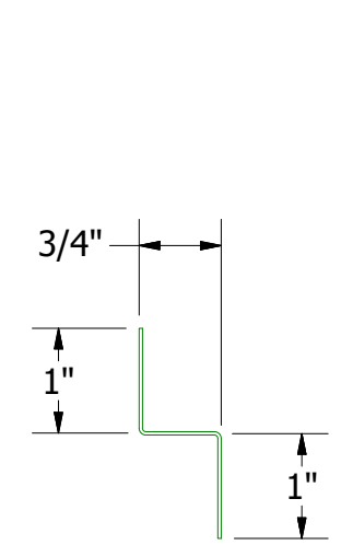
MCA681-Support Z
