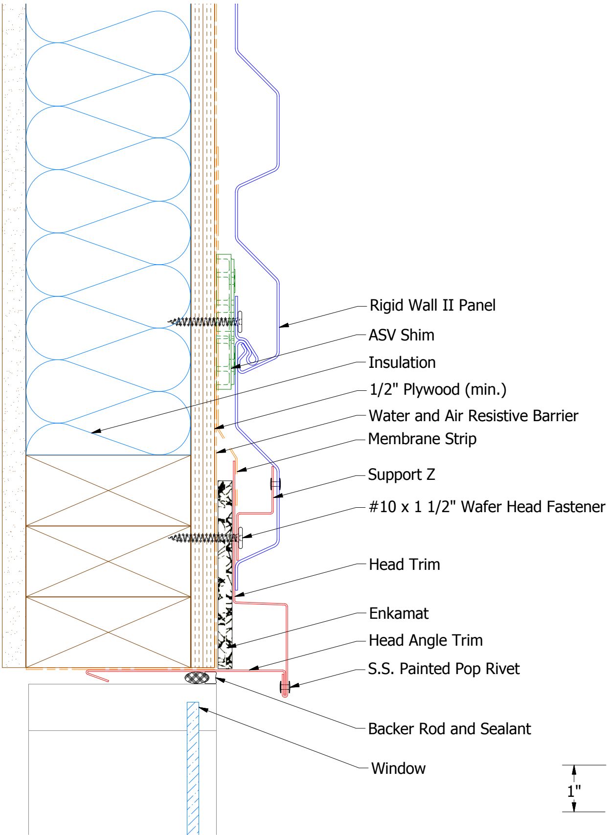
MCA681-Support Z
