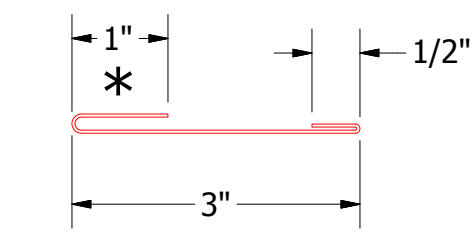
PCA962-Utility Cleat
