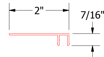
Receiver Extrusion for Jamb Cover
