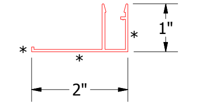
Channel Cover
