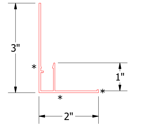
Jamb Cover Extrusion
