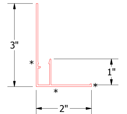
Jamb Cover Extrusion
