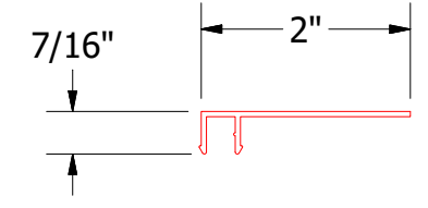
Receiver Extrusion for Jamb Cover
