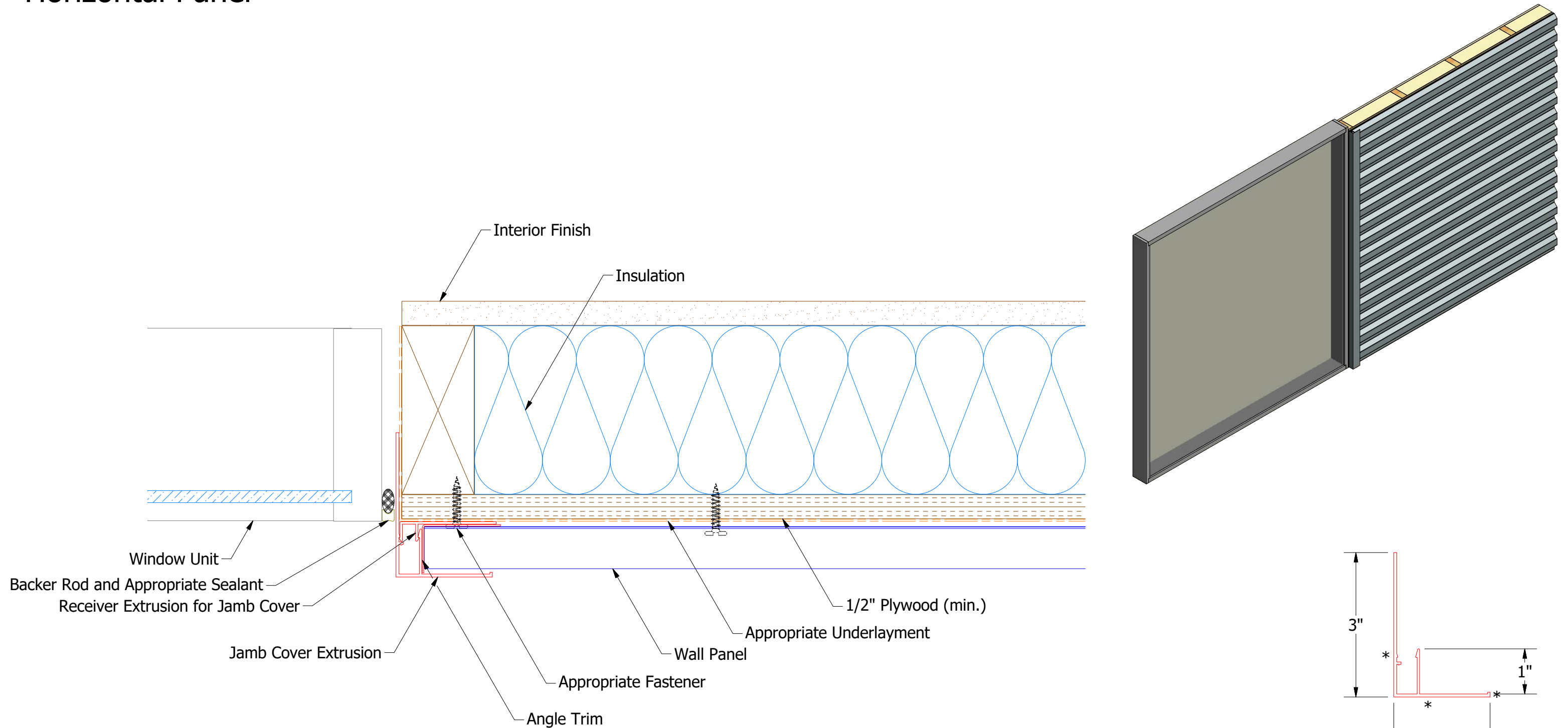
Jamb Cover Extrusion
