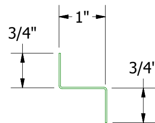
Support Z
