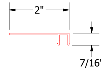
Receiver Extrusion for Channel Cover
