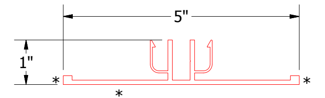
Flush Transition Cover Extrusion
