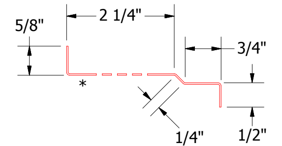
BGA912-Vented Closure Angle
