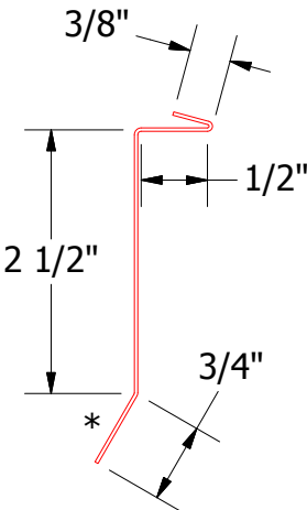
BGA980-Counterflashing
