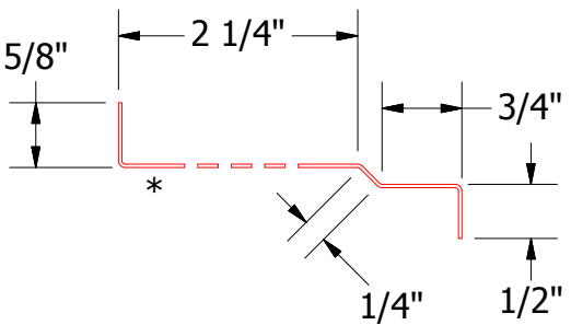
BGA912-Vented Closure Angle
