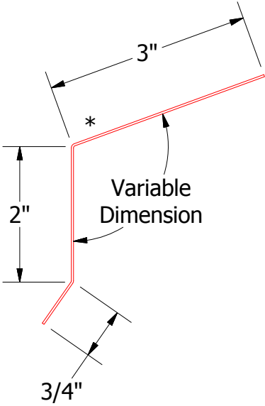
BGA115-Eave Trim
