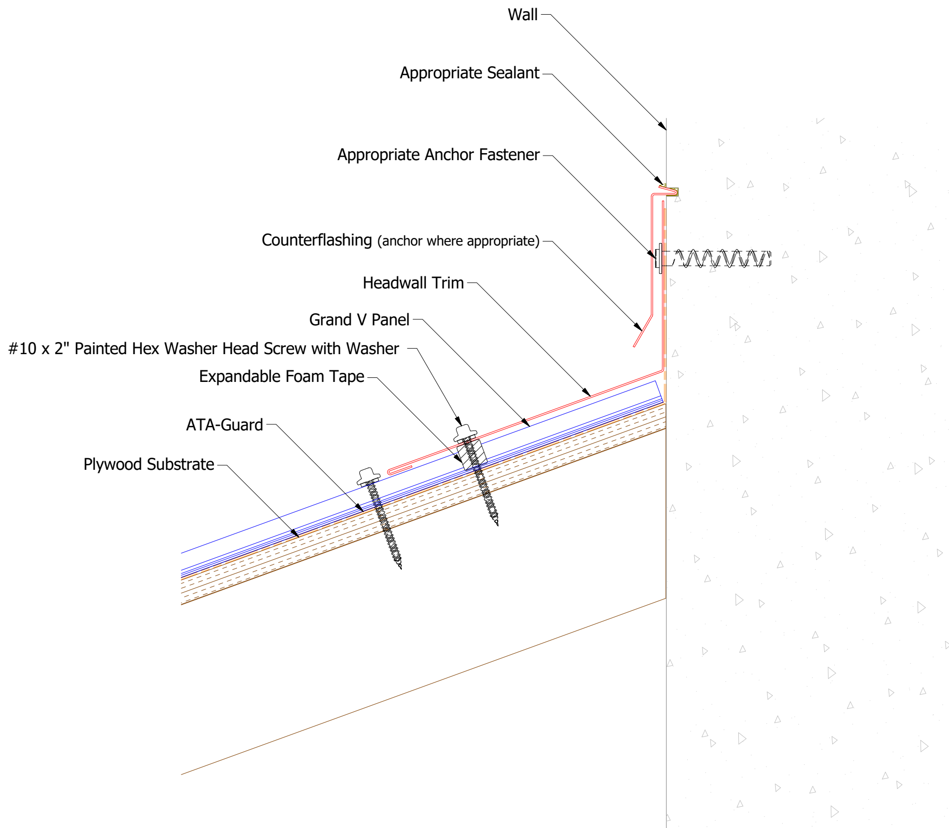
BGA980-Counterflashing
