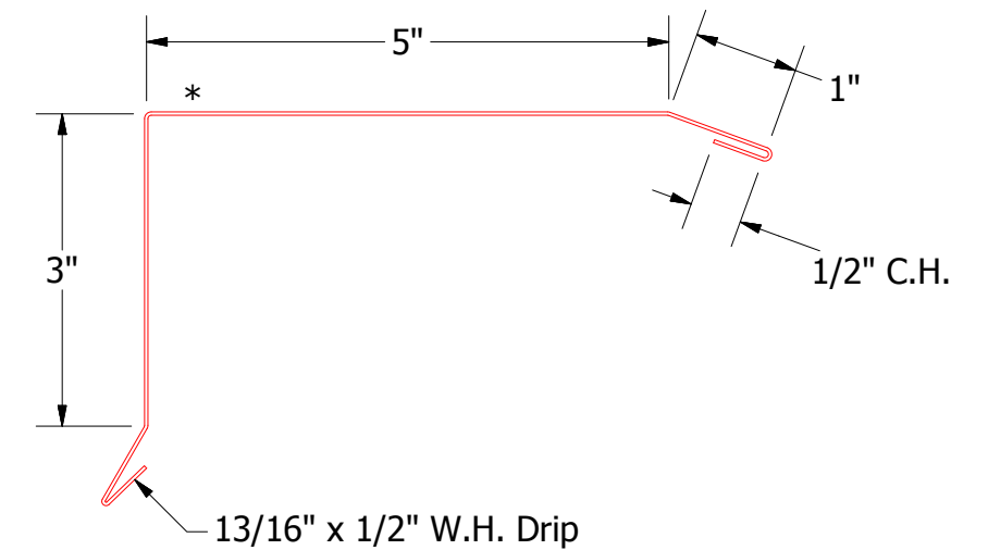
BGA277-Gable Trim - with Angle
