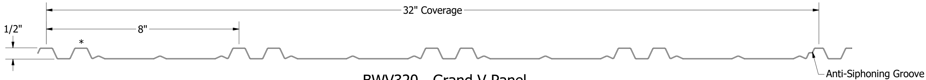
BWV320 - Grand V Panel
