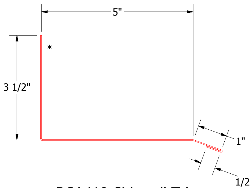
BGA410-Sidewall Trim
