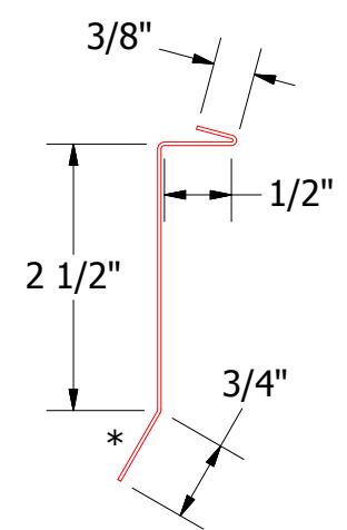
BGA980-Counterflashing
