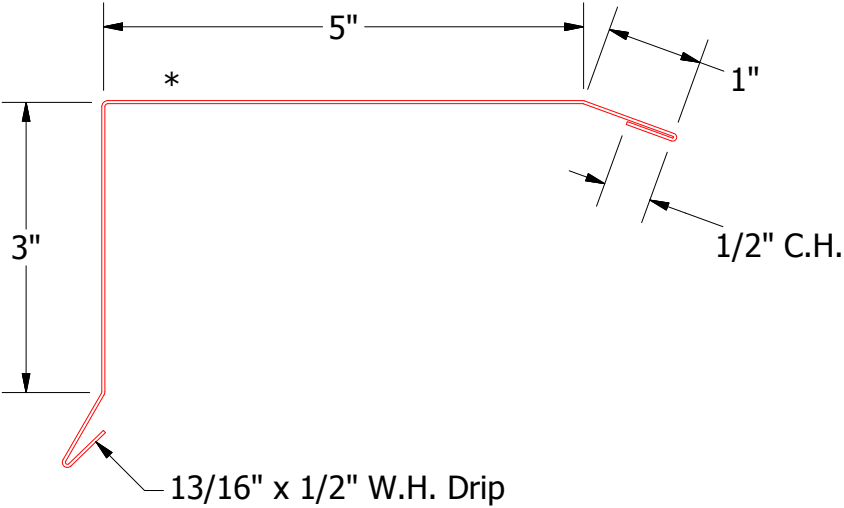
BGA277-Gable Cap - with Angle
